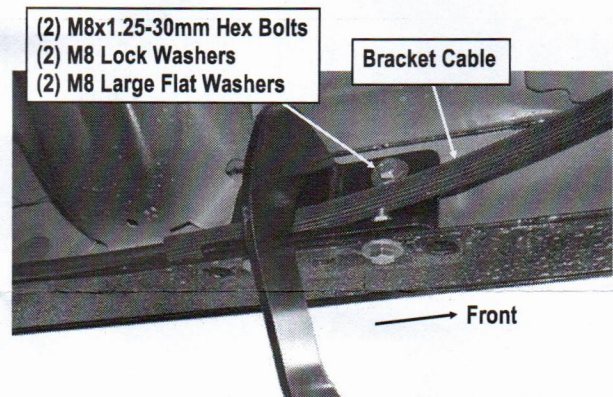
(Fig 3) Driver Front Mounting Bracket Installed
