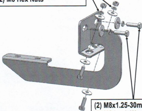
(Fig 4) Driver Front Mounting Bracket Installation
