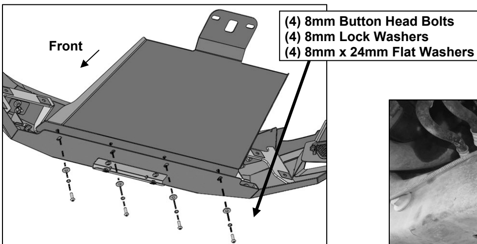
(Fig 3) Attach Skid Plate to the top of the back of the Bumper
