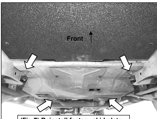
(Fig 7) Reinstall factory skid plate
