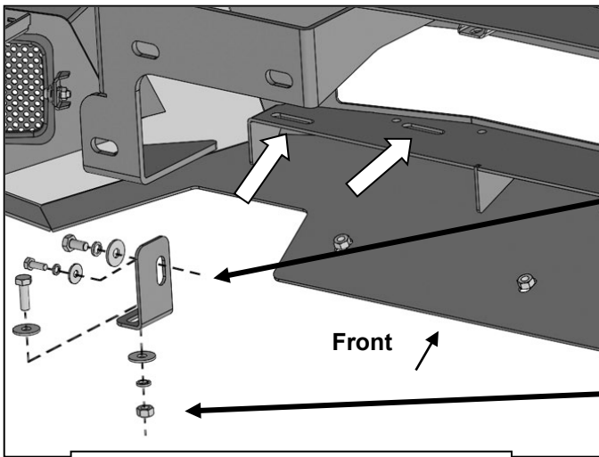
(Fig 10) Driver/left side "L" Bracket attached to the back of the bumper
