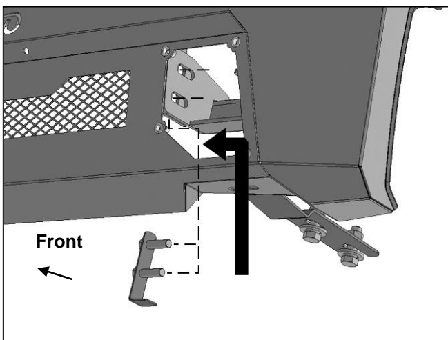
(Fig 15) Insert Double Bolt up and through back of tab on Bumper and Frame Bracket
