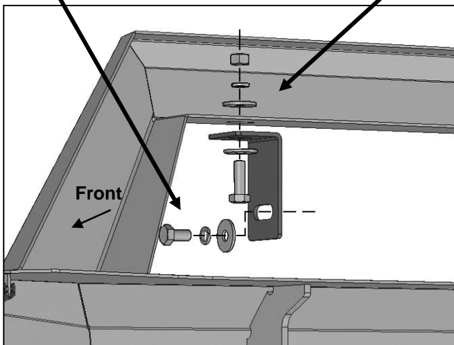
(Fig 18) Attach LED "L" Brackets to bottom of loop. NOTE: Top Light bracket mounting location is designed for 20-24" single or double row bar style light. Flip Brackets around if necessary
