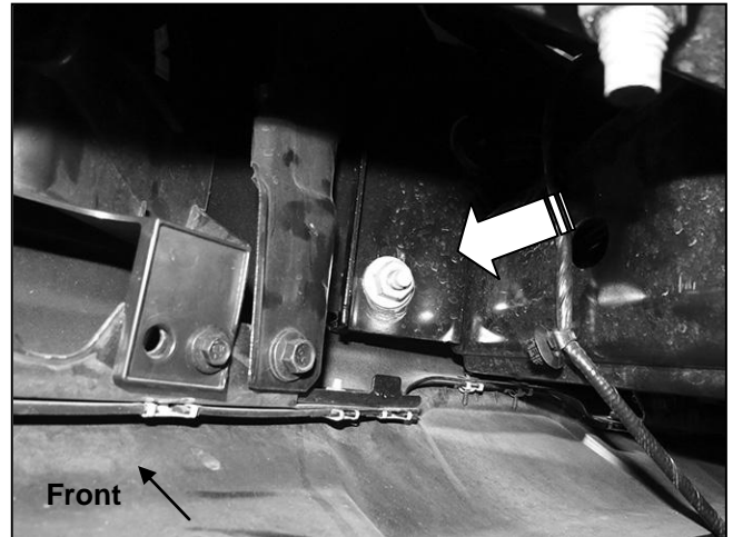
(Fig 10) Models without tow hooks, loosen the front hex nuts to tilt the bumper enough to insert the Double Nut Plates into the end of the frame. Remove factory hex nut (arrow) from back of bumper bracket and tilt bumper forward
