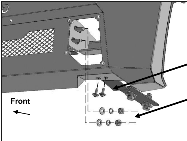
(Fig 16) Attach driver/left side of Bumper to Double Bolt Plate. Attach bottom of Bumper to Support Bracket
