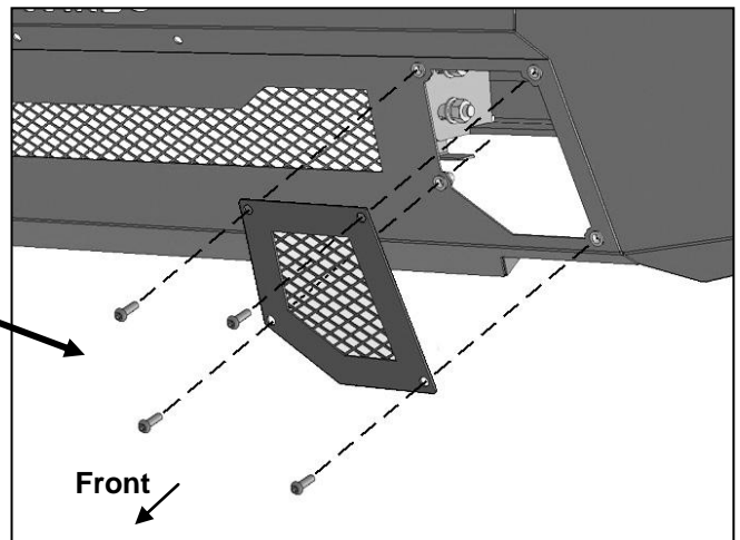
(Fig 17) Attach driver/left Mesh Panel after Bumper has been adjusted and hardware fully tightened
