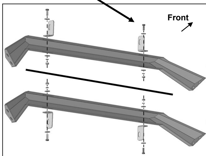
(Fig 2) Attach "L" Brackets to top or bottom of Bull Nose assembly
