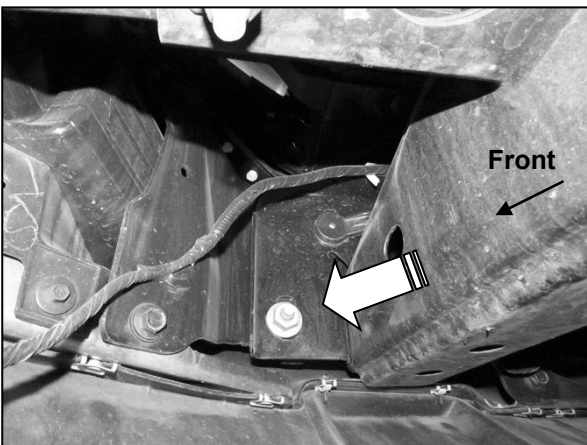
(Fig 5) Remove factory hex nut (arrow) from back of each bumper bracket
