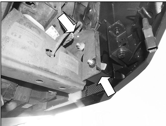
(Fig 17) Reuse factory hex nuts to attach Bumper to ends of frame. Passenger/right side pictured
