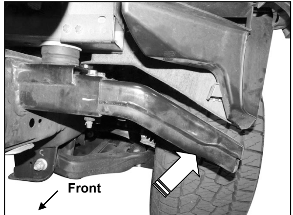
(Fig 7) Remove the factory frame extensions, if equipped (optional)
