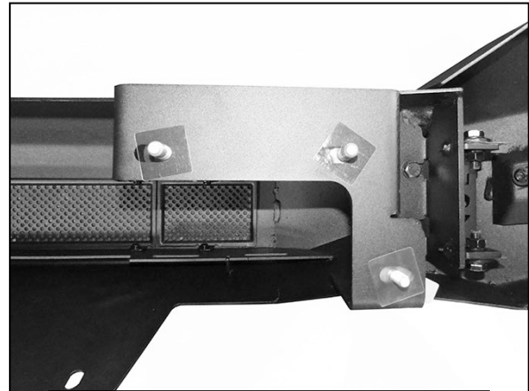
(Fig 16) Factory bolt plates installed
