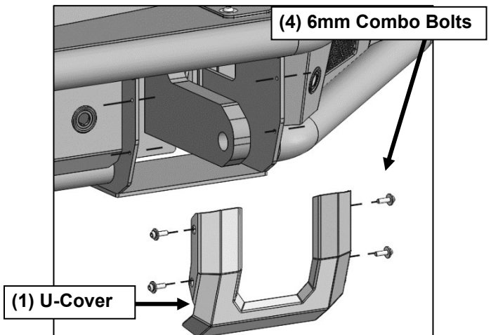
(Fig 27) Once Bumper is fully installed and hardware fully tightened, install U-Covers
