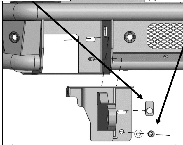
(Fig 19) Attach Shackle Mount to threaded stud on Bumper. Insert Single Bolt Plate through top inner mounting slot
