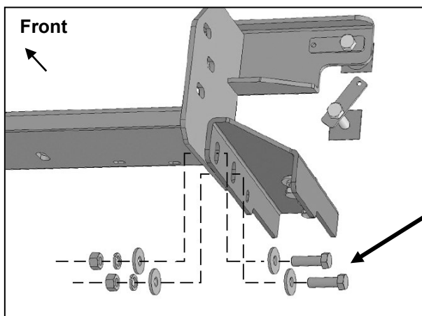
(Fig 24) Attach driver/left Support Bracket to outside of Winch Tray
