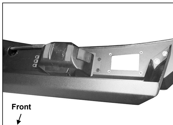
(Fig 31) Attach Relocation Bracket to winch control unit. Attach assembly to top of Bumper
