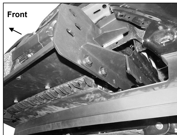
(Fig 25) Bumper, Winch Tray assembly and air dam installed
