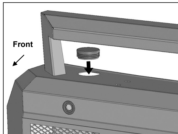
(Fig 27) Models without winch, insert Plug
