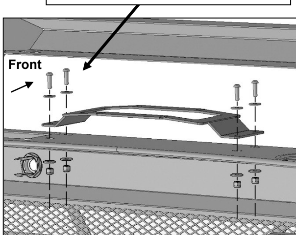
(Fig 30) Attach Relocation Bracket to winch control unit. Attach assembly to top of Bumper
