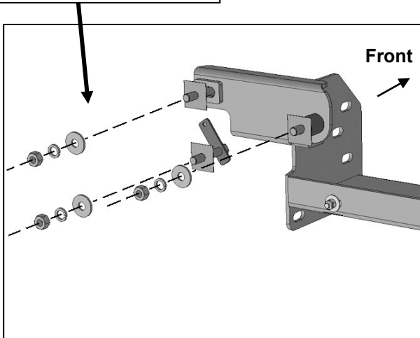
(Fig 20) Attach factory bumper with inner Winch Tray Bracket Assembly to end of frame
