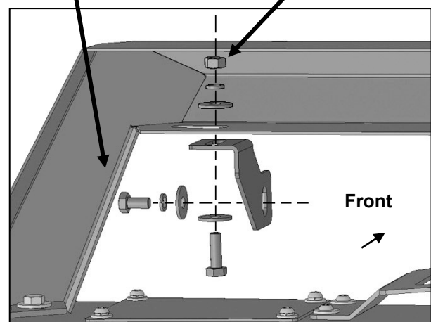
(Fig 35) Attach LED "L" Brackets to bottom of hoop
