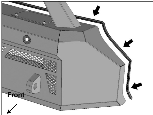
(Fig 26) Push Edge Trim onto inner edge of CS1 Bumper. Cut to fit Bumper
