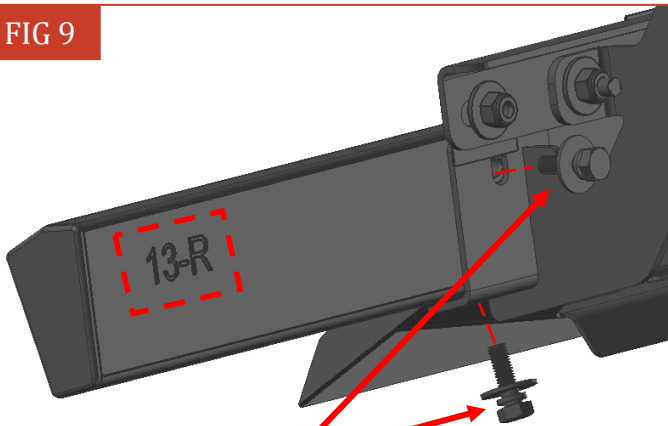
(Fig 9) Attach the Passenger/Right Running Board to the Mounting Brackets
