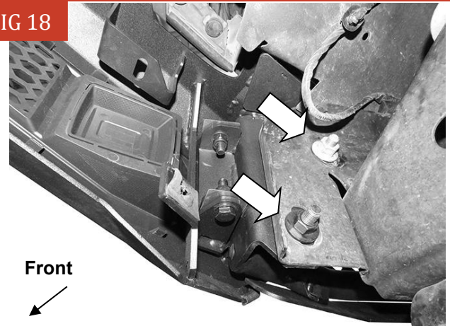
(Fig 18) Reuse factory hex nuts (arrows) to attach Bumper to end of the frame (driver/left installation pictured)
