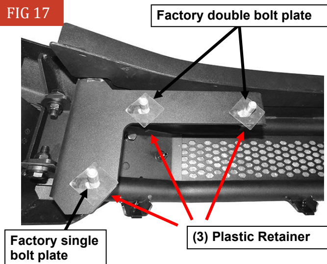
(Fig 17) Use the included (3) Plastic Retainers to hold the factory bolt plates in place on the back of the Bumper (driver/left side pictured)
