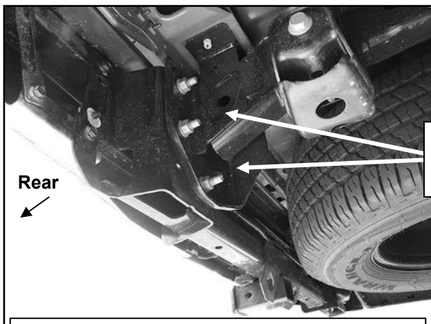
(Fig 3) Note bumper with "HD" tow package receiver hitch integrated into bumper bracket
