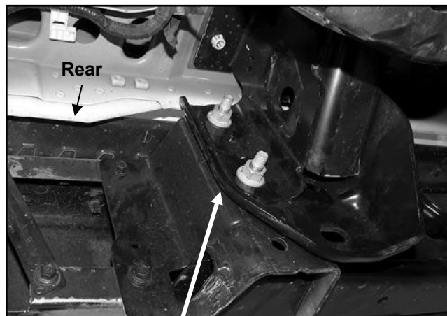
(Fig 4) Remove the factory hex nuts attaching bumper assembly to frame. STD tow package model pictured (no receiver hitch)
