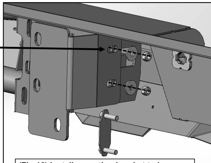
(Fig 16) Install mounting bracket to bumper
