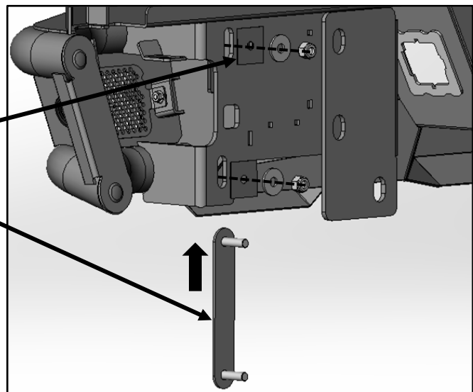
(Fig 14) HW used to mount bumper to hitch
