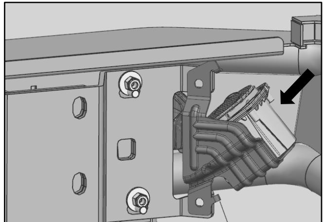
(Fig 20) Install PAS using OEM clip nuts and bolts
