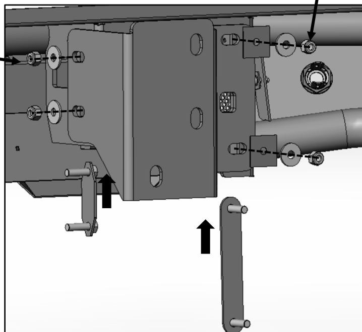
(Fig 18) HW used to mount bumper to mounting brackets
