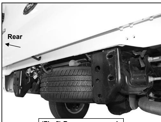
(Fig 5) Bumper removed
