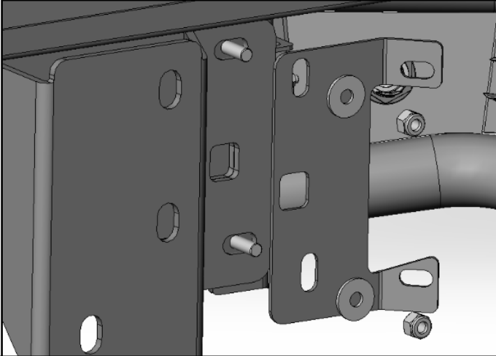
(Fig 19) HW used to mount PAS bracket to mounting brackets
